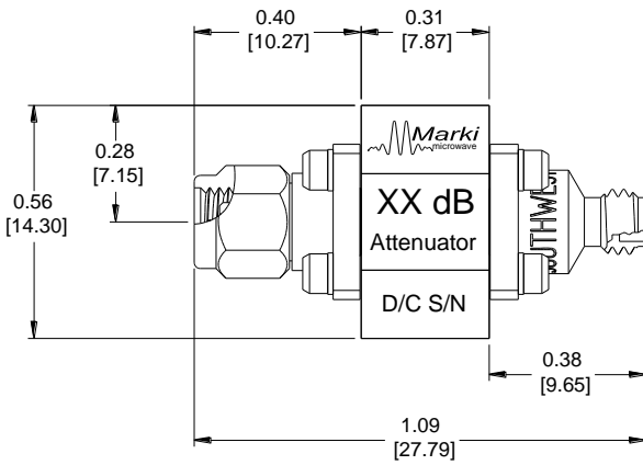
Topside View
