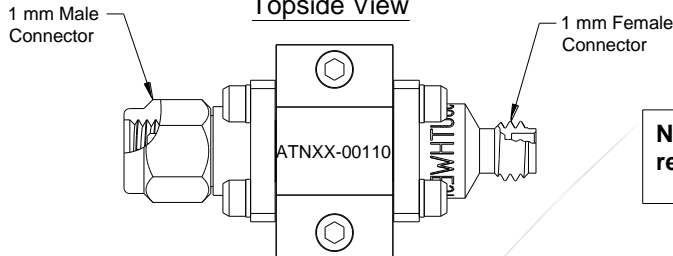
Topside View
