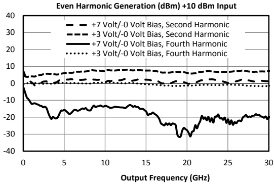
Typical Performance: Positive Only (+3 to +7V) Bias (Pin 16 Output), Grounded Gate (Pin 11), continued
