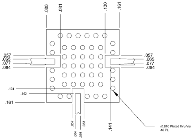
QFN-Package Surface-Mount Landing Pattern
