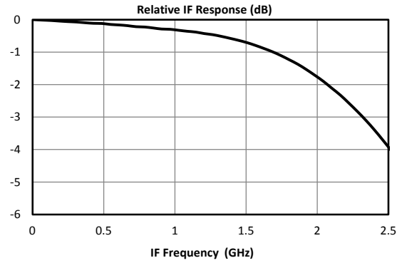
Typical Performance
