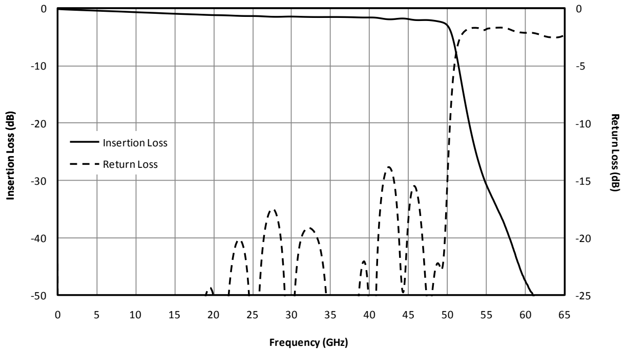
Fig. 1. Magnitude response for a typical FLP-5000.
