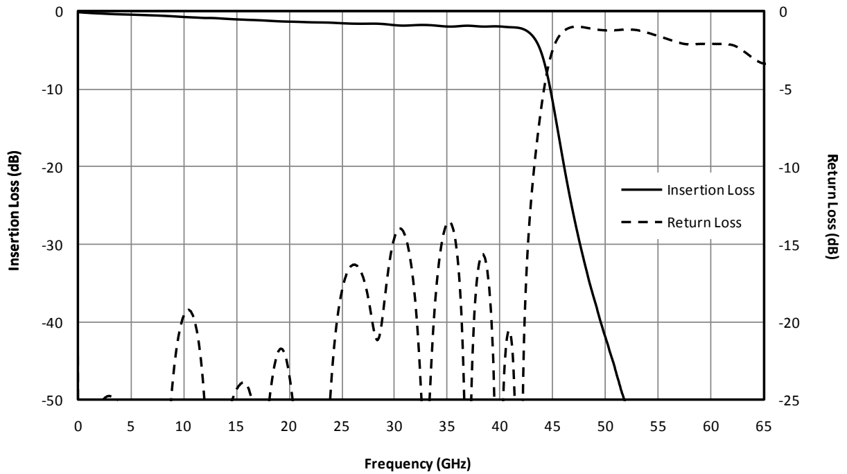
Fig. 1. Magnitude response for a typical FLP-4300.
