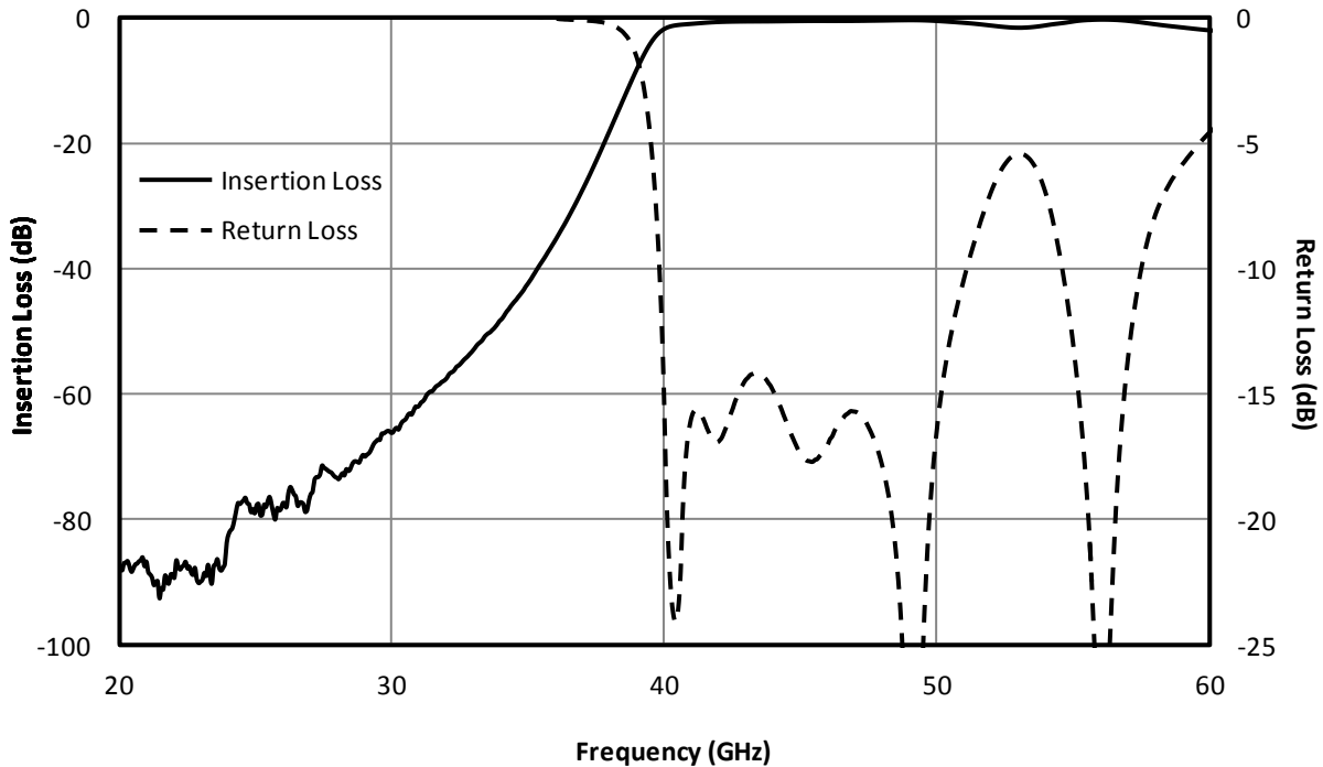
Fig. 1. Magnitude response for a typical FH-4000 Filter.
