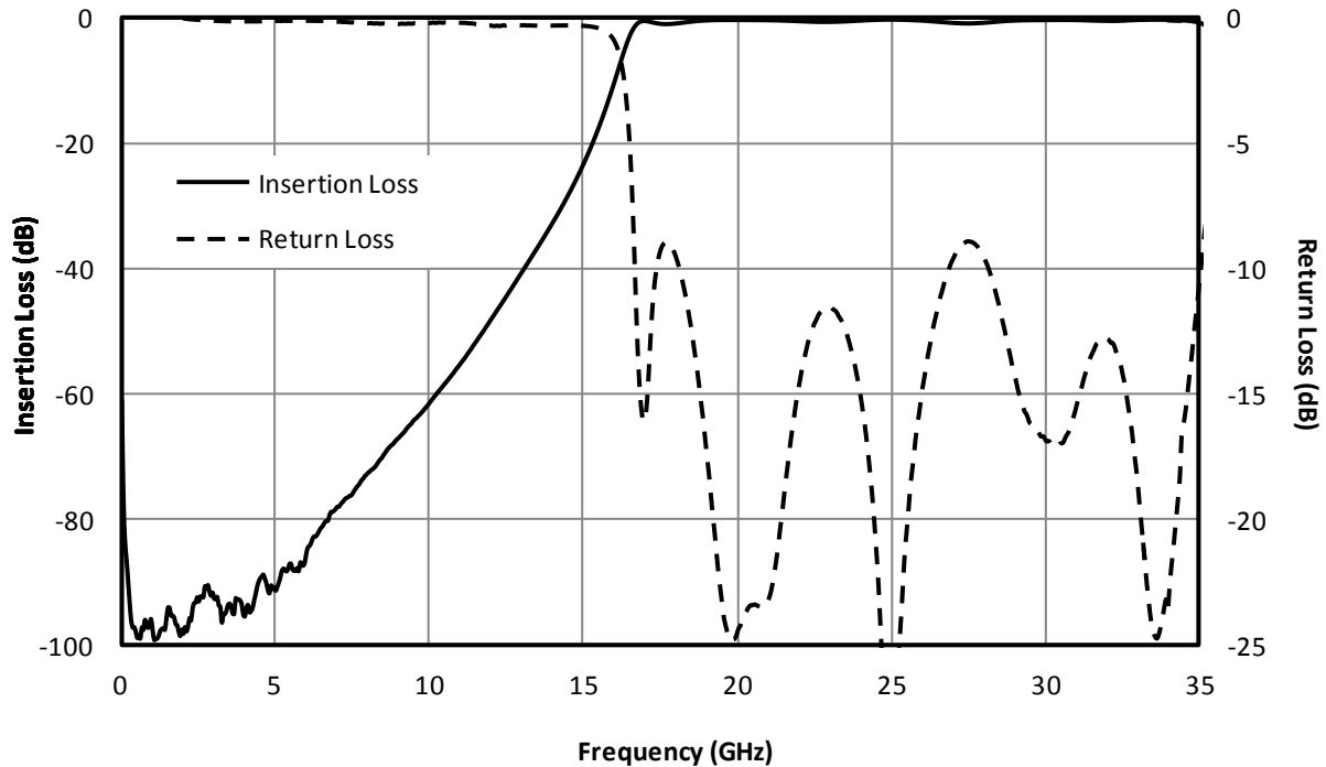
Fig. 1. Magnitude response for a typical FH-1700 Filter.
