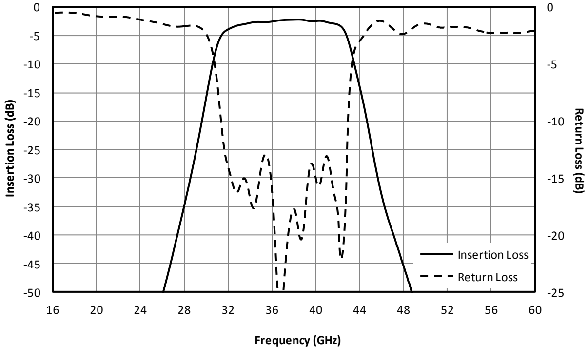
Fig. 1. Magnitude response for a typical FB-3700.
