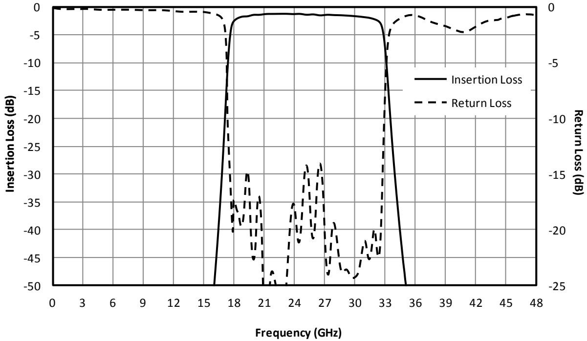
Fig. 1. Magnitude response for a typical FB-2500.
