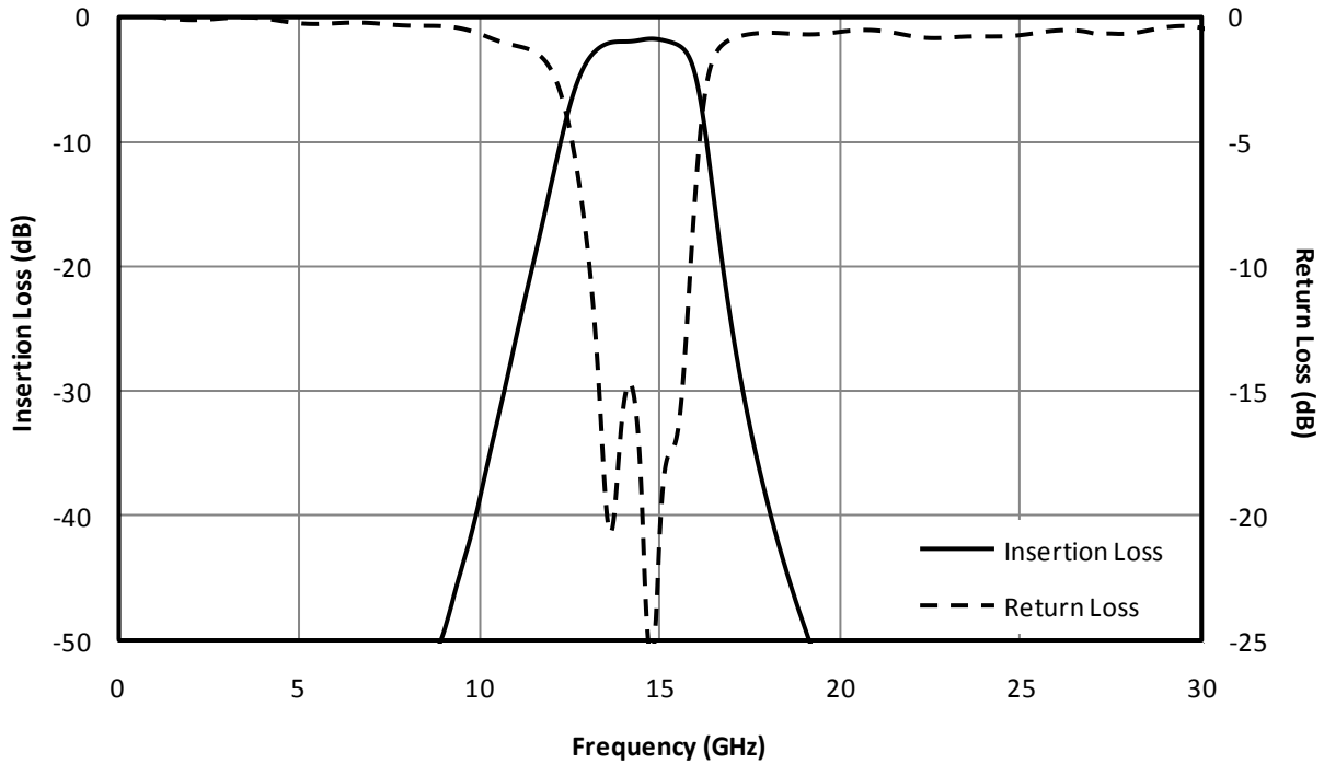
Fig. 1. Magnitude response for a typical FB-1445SM, measured in a connectorized fixture.
