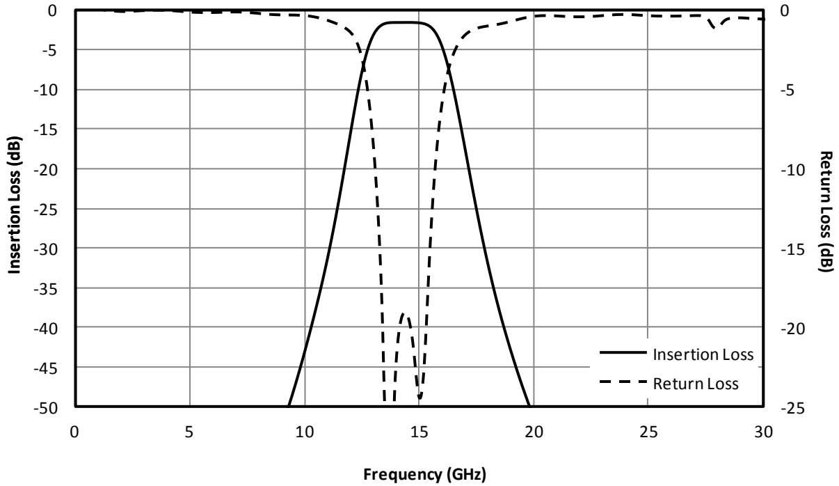
Fig. 1. Magnitude response for a typical FB-1445.
