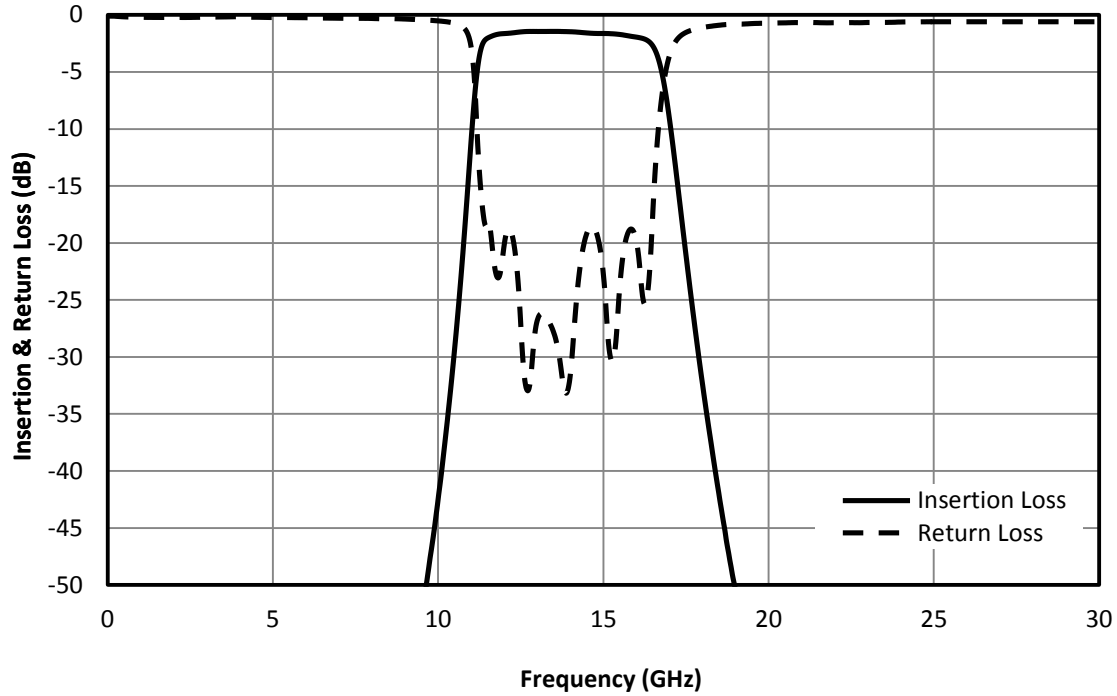
Fig. 1. Magnitude response for a typical FB-1385.
