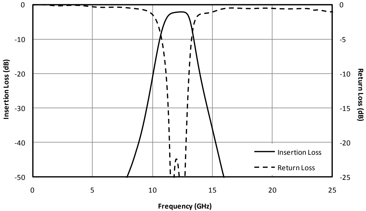
Fig. 1. Magnitude response for a typical FB-1215SM, measured in a connectorized fixture.
