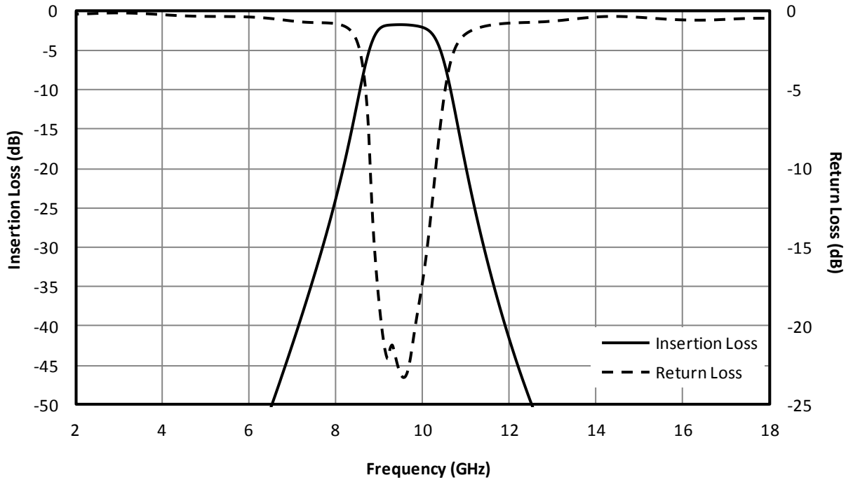
Fig. 1. Magnitude response for a typical FB-0955.
