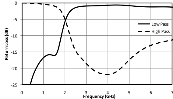
Fig. 3. Return loss.
