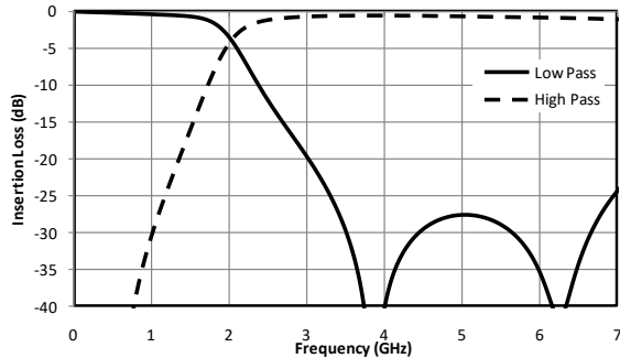
Fig. 2. Insertion loss.
