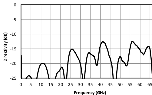
Fig. 4. Typical directivity.
