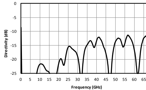
Fig. 4. Typical directivity.
