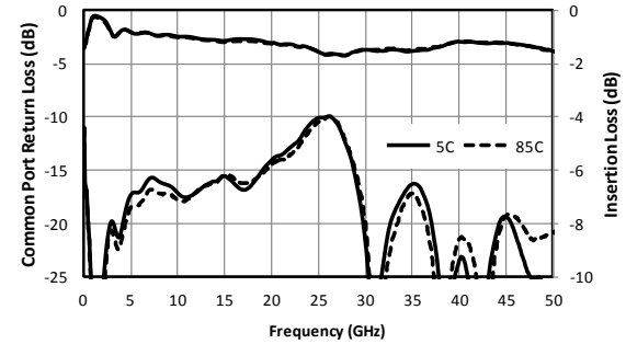
Fig. 9. Performance over temperature
