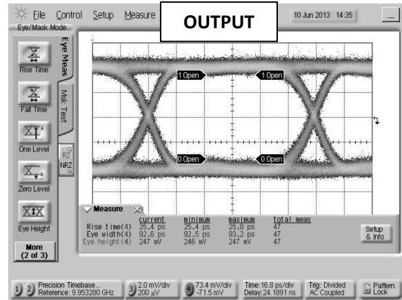
Fig. 7. Oscilloscope measurements of the BTN2-0050 with a 10Gb/s PRBS pattern. Eye diagrams are taken with a 2 31 -1 PRBS input demonstrating minimal eye distortion/closure afforded by the extremely low frequency operation of the bias tee.
