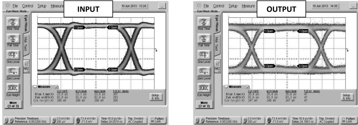
Fig. 7. Oscilloscope measurements of the BTN2-0040 with a 10Gb/s PRBS pattern. Eye diagrams are taken with a 2 31 -1 PRBS input demonstrating minimal eye distortion/closure afforded by the extremely low frequency operation of the bias tee.
