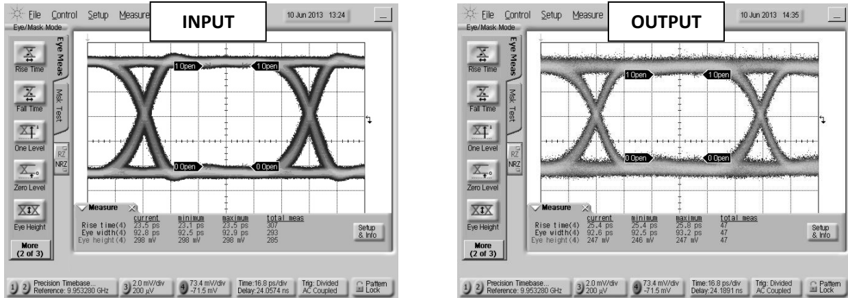
Fig. 10. Oscilloscope measurements of the BTN2-0040 with a 10Gb/s PRBS pattern. Eye diagrams are taken with a 2^{31}-1 PRBS input demonstrating minimal eye distortion/closure afforded by the extremely low frequency operation of the bias tee.
