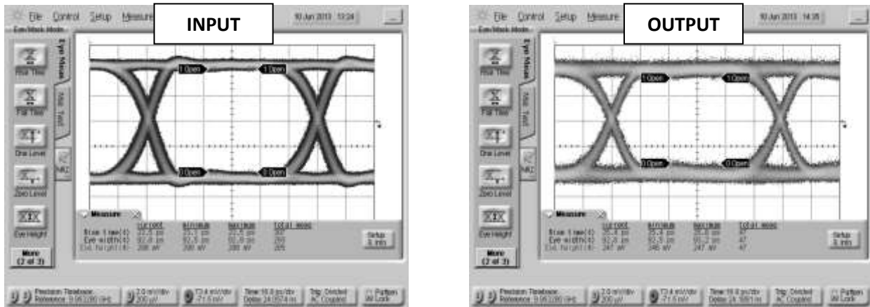
Fig. 7. Oscilloscope measurements of the BTN2-0040 with a 10Gb/s PRBS pattern. Eye diagrams are taken with a 2^{31}-1 PRBS input demonstrating minimal eye distortion/closure afforded by the extremely low frequency operation of the bias tee.
