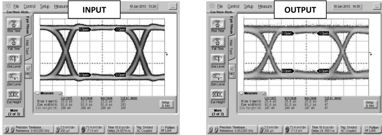
Fig. 7. Oscilloscope measurements of the BTN2-0026 with a 10Gb/s PRBS pattern. Eye diagrams are taken with a 2 31 -1 PRBS input demonstrating minimal eye distortion/closure afforded by the extremely low frequency operation of the bias tee.
