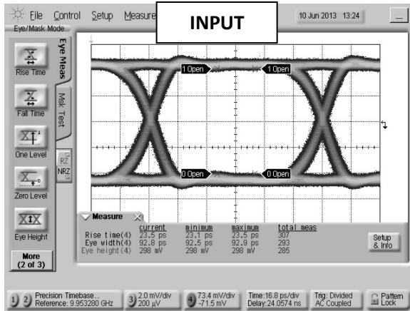
Fig. 10. Oscilloscope measurements of the BTN2-0026 with a 10Gb/s PRBS pattern. Eye diagrams are taken with a 2^{31}-1 PRBS input demonstrating minimal eye distortion/closure afforded by the extremely low frequency operation of the bias tee.
