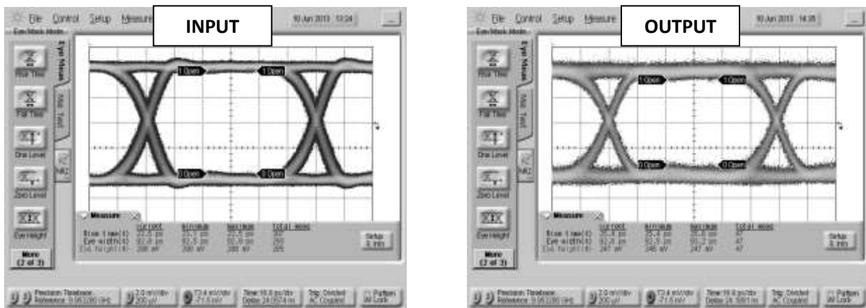
Fig. 7. Oscilloscope measurements of the BTN2-0026 with a 10Gb/s PRBS pattern. Eye diagrams are taken with a 2^{31}-1 PRBS input demonstrating minimal eye distortion/closure afforded by the extremely low frequency operation of the bias tee.
