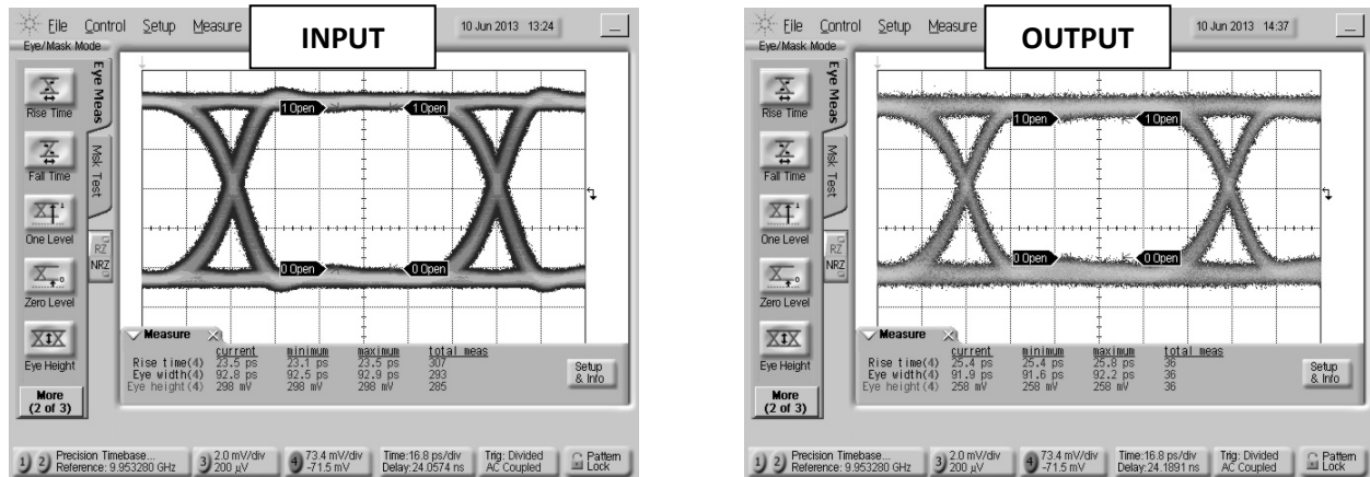
Fig. 10. Oscilloscope measurements of the BTN1-0040 with a 10Gb/s PRBS pattern. Eye diagrams are taken with a 2^{31}-1 PRBS input demonstrating minimal eye distortion/closure afforded by the extremely low frequency operation of the bias tee.
