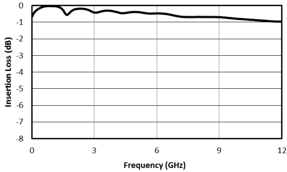
Fig. 1. Insertion loss.
