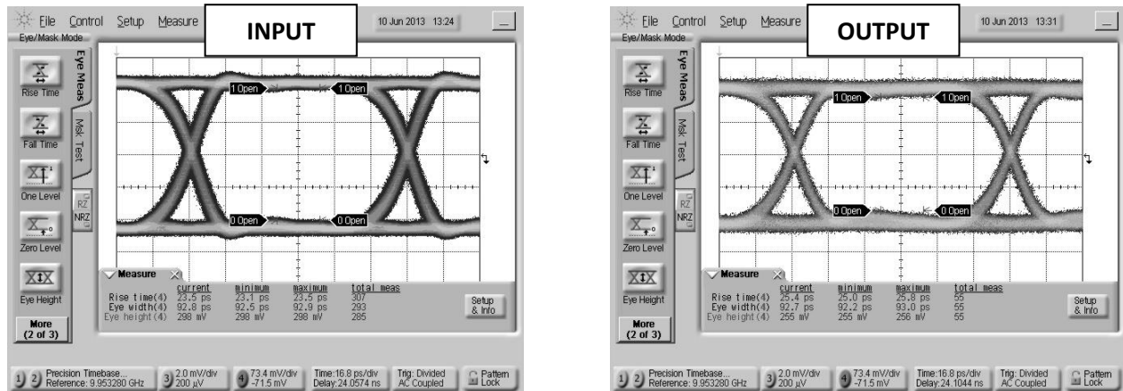
Fig. 13. Oscilloscope measurements of the BT2-0040 with a 10Gb/s PRBS pattern. Eye diagrams are taken with a 2^{31}-1 PRBS input demonstrating minimal eye distortion/closure afforded by the extremely low frequency operation of the bias tee.
