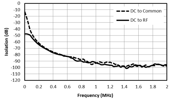
Fig. 5. Low frequency isolation.
