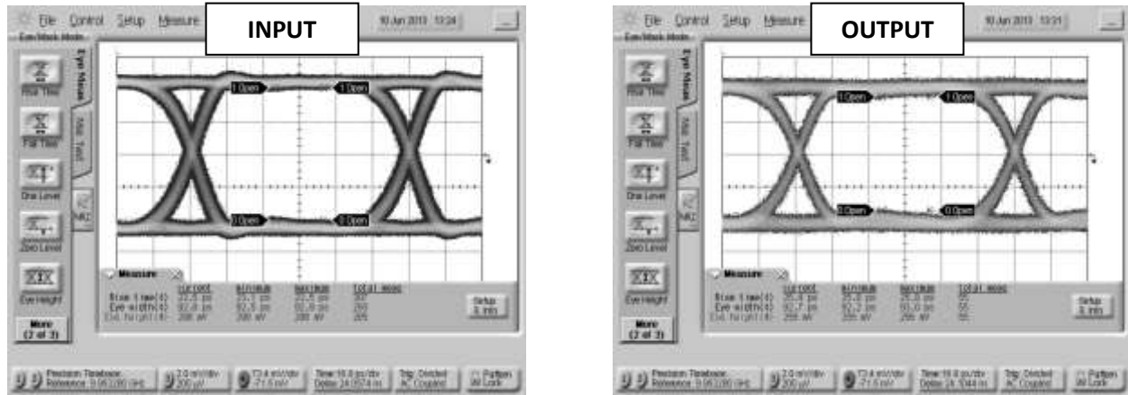
Fig. 7. Oscilloscope measurements of the BT2-0026 with a 10Gb/s PRBS pattern. Eye diagrams are taken with a 2^{31}-1 PRBS input demonstrating minimal eye distortion/closure afforded by the extremely low frequency operation of the bias tee.
