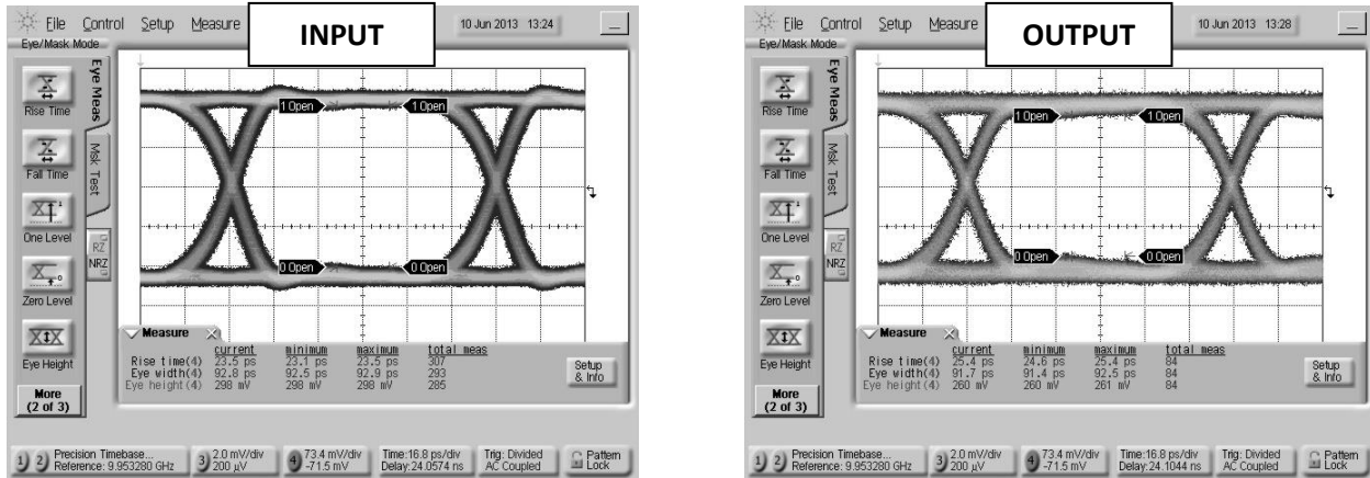
Fig. 13. Oscilloscope measurements of the BT1-0050 with a 10Gb/s PRBS pattern. Eye diagrams are taken with a 2^{31}-1 PRBS input demonstrating minimal eye distortion/closure afforded by the extremely low frequency operation of the bias tee.
