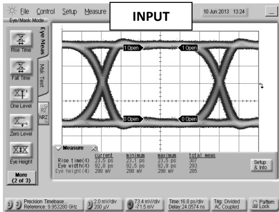
Fig. 7. Oscilloscope measurements of the BT1-0050 with a 10Gb/s PRBS pattern. Eye diagrams are taken with a 2^{31}-1 PRBS input demonstrating minimal eye distortion/closure afforded by the extremely low frequency operation of the bias tee.
