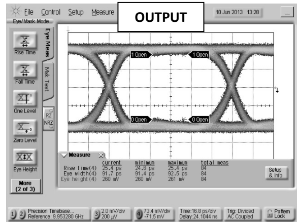
Fig. 7. Oscilloscope measurements of the BT1-0050 with a 10Gb/s PRBS pattern. Eye diagrams are taken with a 2^{31}-1 PRBS input demonstrating minimal eye distortion/closure afforded by the extremely low frequency operation of the bias tee.
