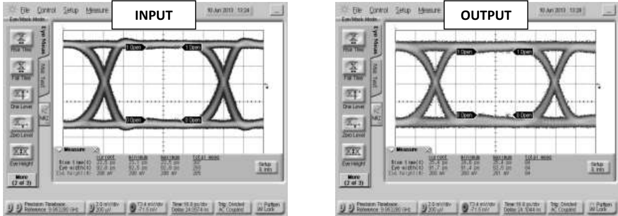
Fig. 7. Oscilloscope measurements of the BT1-0050 with a 10Gb/s PRBS pattern. Eye diagrams are taken with a 2^{31}-1 PRBS input demonstrating minimal eye distortion/closure afforded by the extremely low frequency operation of the bias tee.
