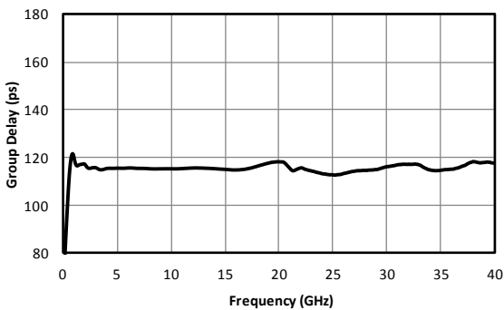
Fig. 8. Group delay.
