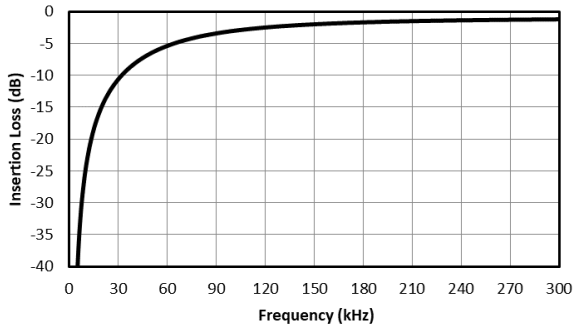
Fig. 4. Low frequency RF response.
