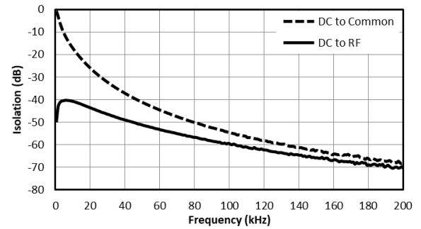
Fig. 7. Near DC isolation
