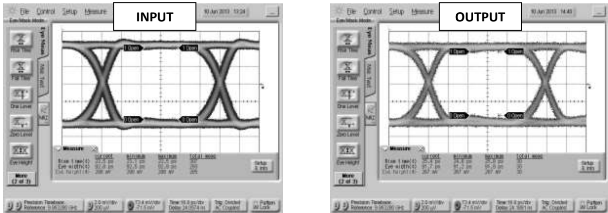
Fig. 7. Oscilloscope measurements of the BT-0065 with a 10Gb/s PRBS pattern. Eye diagrams are taken with a 2^{31}-1 PRBS input demonstrating minimal eye distortion/closure afforded by the extremely low frequency operation of the bias tee.
