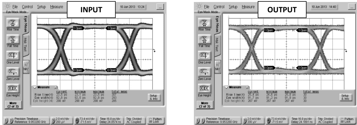
Fig. 13. Oscilloscope measurements of the BT-0040 with a 10Gb/s PRBS pattern. Eye diagrams are taken with a 2^{31}-1 PRBS input demonstrating minimal eye distortion/closure afforded by the extremely low frequency operation of the bias tee.
