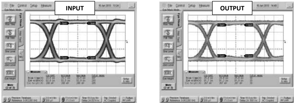
Fig. 7. Oscilloscope measurements of the BT-0040 with a 10Gb/s PRBS pattern. Eye diagrams are taken with a 2^{31}-1 PRBS input demonstrating minimal eye distortion/closure afforded by the extremely low frequency operation of the bias tee.
