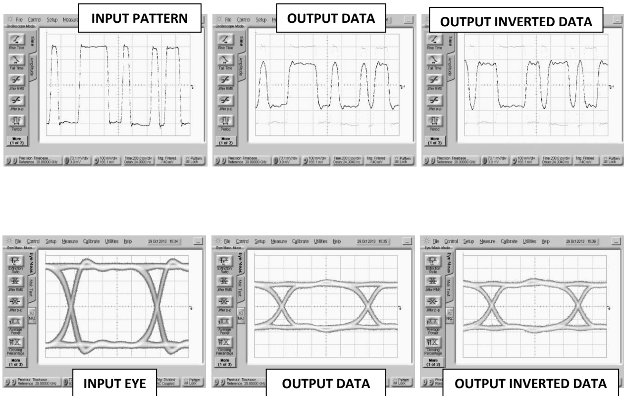
Fig. 1. Oscilloscope measurements of the BALH-0009SMG with a 10 Gb/s PRBS pattern. Bit pattern is measured with a 2^7-1 PRBS input demonstrating extremely good pulse fidelity for both inverted and non-inverted output. Eye diagrams are taken with a 2^{31}-1 PRBS input demonstrating minimal eye distortion/closure afforded by the extremely low frequency operation of the balun (<500 kHz).
