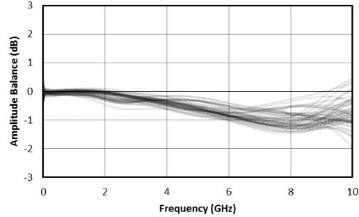
Fig. 13. Amplitude balance between output ports.
