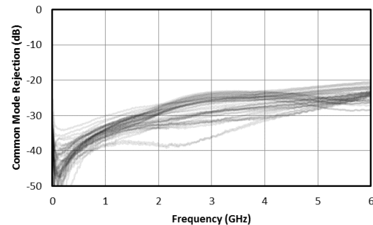
Fig.17. Common mode rejection.
