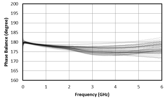
Fig. 15. Phase balance between output ports.
