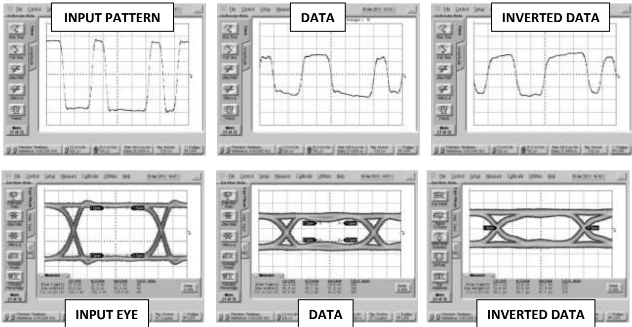
Fig. 6. Oscilloscope measurements of the BALH-0006 with a 10 Gb/s PRBS pattern. Bit pattern is measured with a 2^7-1 PRBS input demonstrating extremely good pulse fidelity for both inverted and non-inverted output. Eye diagrams are taken with a 2^{31}-1 PRBS input demonstrating minimal eye distortion/closure afforded by the extremely low frequency operation of the balun (<200 kHz).
