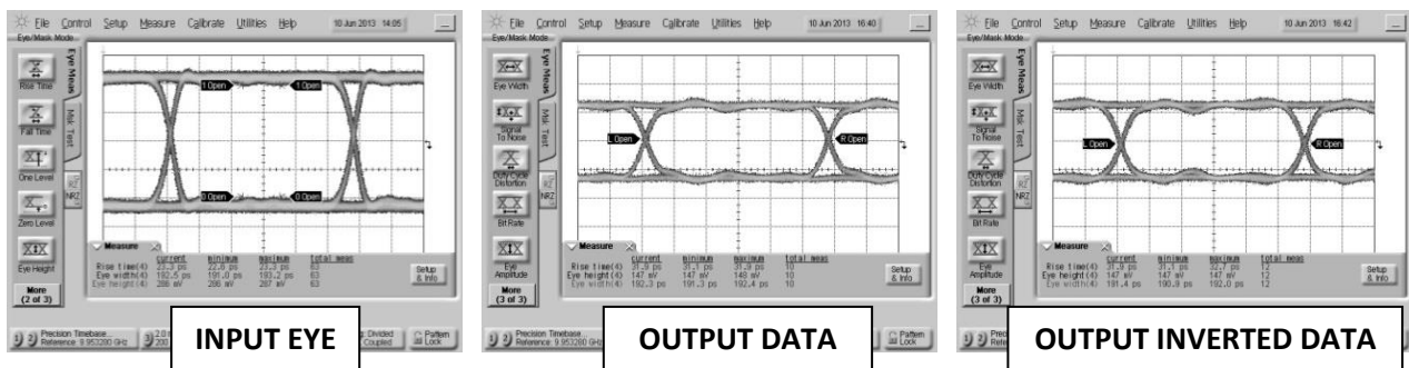
Fig. 1. Oscilloscope measurements of the BALH-0003SMG with a 5 Gb/s PRBS pattern. Bit pattern is measured with a 2^7-1 PRBS input demonstrating extremely good pulse fidelity for both inverted and non-inverted output. Eye diagrams are taken with a 2^{31}-1 PRBS input demonstrating minimal eye distortion/closure afforded by the extremely low frequency operation of the balun (<500 kHz).
