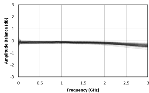
Fig. 13. Amplitude balance, 50 unit spread.
