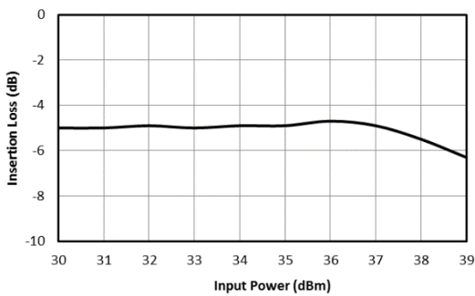
Fig. 18. Output Compression
