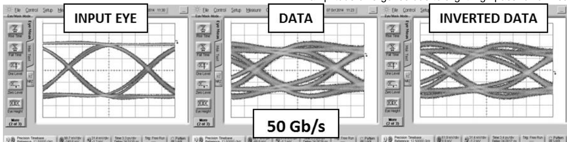
Oscilloscope measurements of the BAL-0050 with a 50 Gb/s PRBS pattern in single ended-to-differential mode. Eye diagrams are taken with a 231-1 PRBS input demonstrating minimal eye distortion/closure afforded by the extremely low frequency operation of the balun (<300 kHz).
