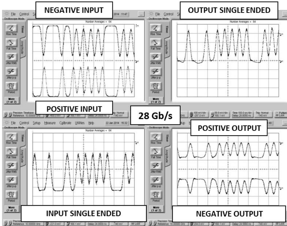
Oscilloscope measurements of the BAL-0026 with a 28 Gb/s PRBS pattern. Bit pattern is measured with a 2^7-1 PRBS input demonstrating extremely good pulse fidelity for both differential-to-single ended and single ended to differential mode conversions. Apparent baseline wander in differential-to-single ended is due to low pass filtering by test cables.
