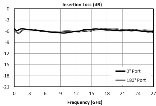
Single ended to differential
