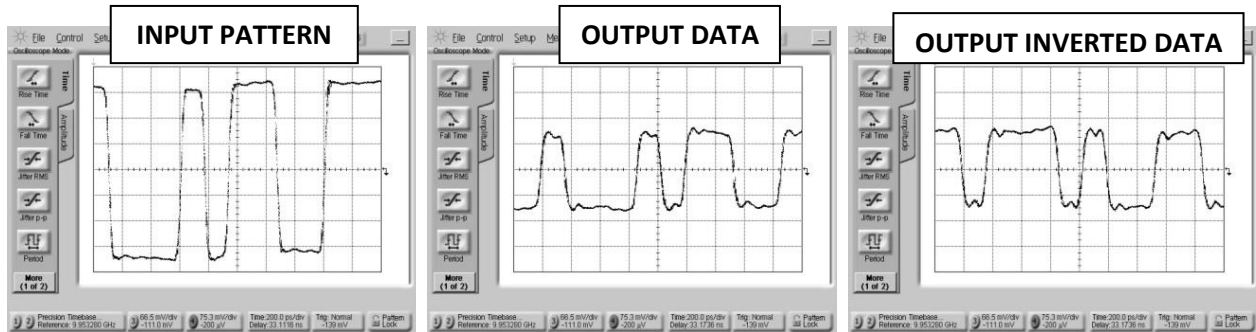
Fig. 5. Common mode rejection.
