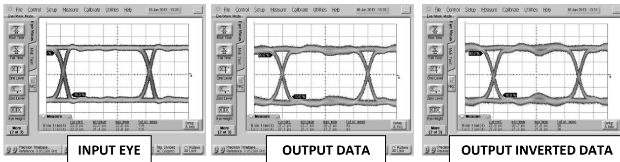
Fig. 6. Oscilloscope measurements of the BAL-0006SMG with a 6 Gb/s PRBS pattern. Bit pattern is measured with a 2^7-1 PRBS input demonstrating extremely good pulse fidelity for both inverted and non-inverted output. Eye diagrams are taken with a 2^{31}-1 PRBS input demonstrating minimal eye distortion/closure afforded by the extremely low frequency operation of the balun (<500 kHz).
