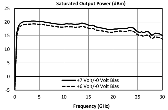
Typical Performance: Positive Only (+6 to +7V) Bias (Pin 20), Grounded Gate (Pin 11)
