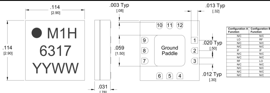
Outline Drawing – 3mm QFN package
