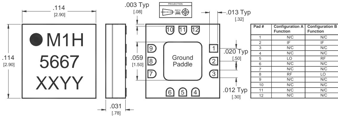
Outline Drawing – QFN package
