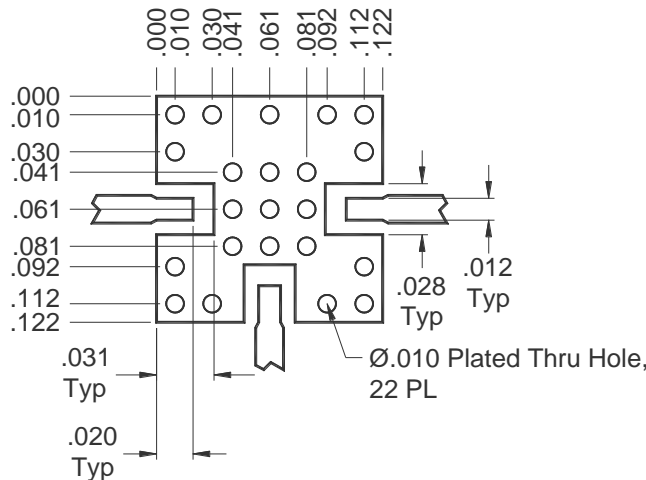
QFN-Package Surface-Mount Landing Pattern
