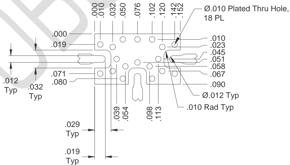
Outline Drawing – SM-2 Package
