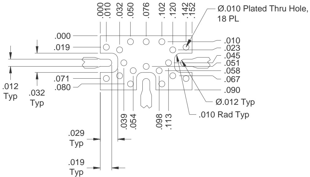
SM-2 Package Surface-Mount System Circuit Footprint
