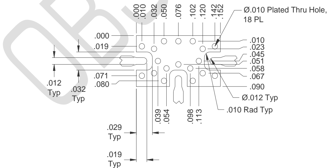
Outline Drawing – SM-2 and SM-1 Packages
